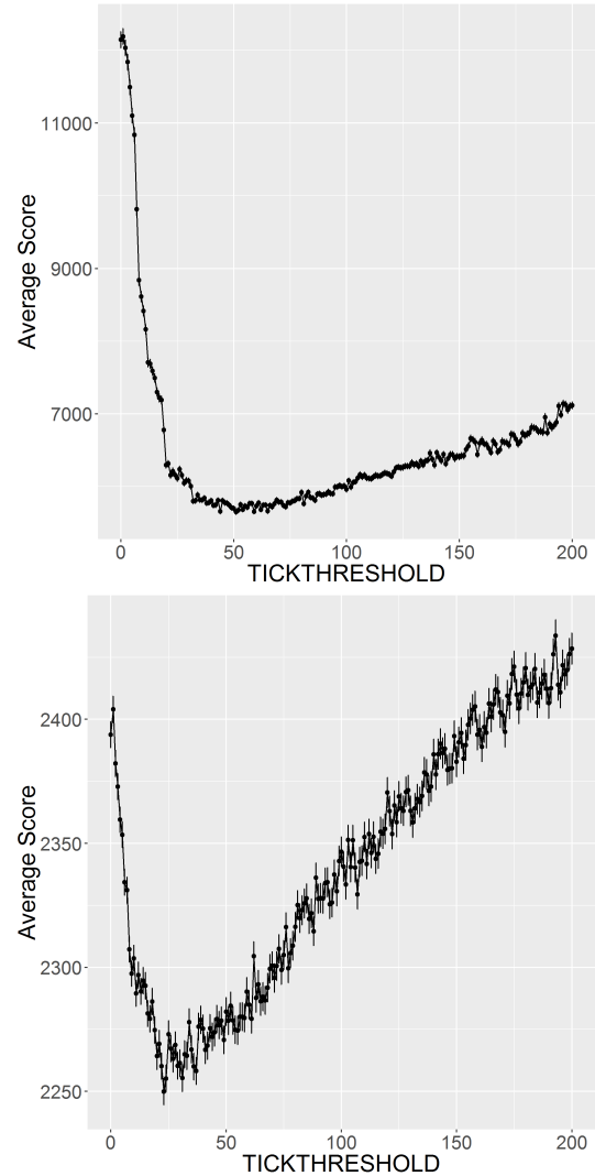
Figure 4. Tuning results of POGC against COP(Top) and POP(Bottom) both with error bars.
